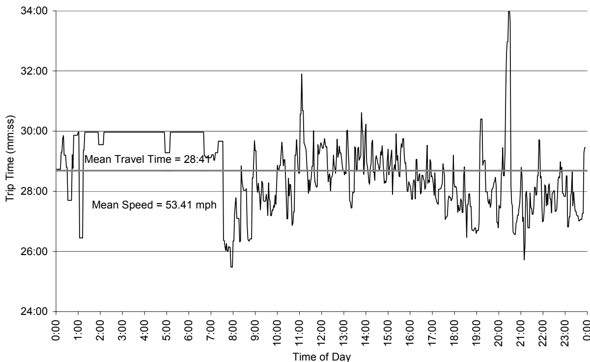
FIGURE 3 Frontier Travel Times, Raw Data: Westbound, Valley Junction to Lincoln City
