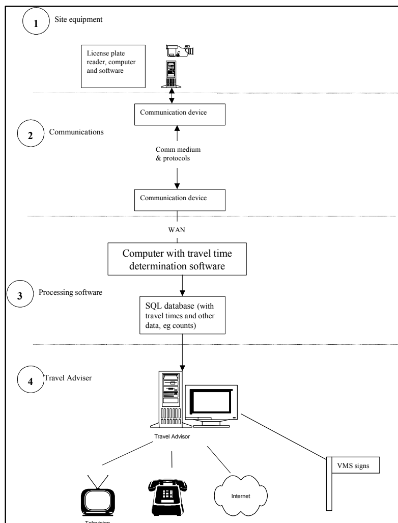
FIGURE 2 Travel Time Estimation System
