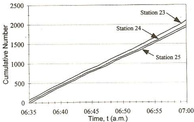
FIGURE 8 Arrival curves constructed from "raw" data, Day 1.
