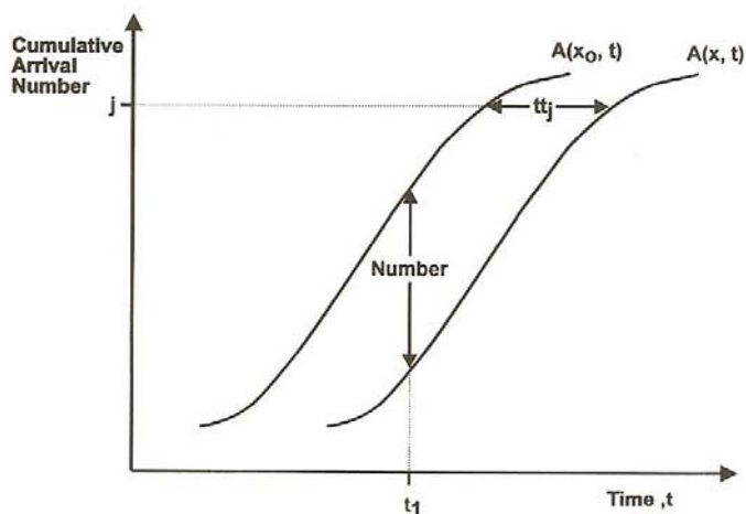
FIGURE 2 Input-output diagram.
