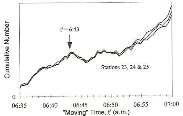
FIGURE 9 Arrival curves in moving time with background flow removed, Day 1.
