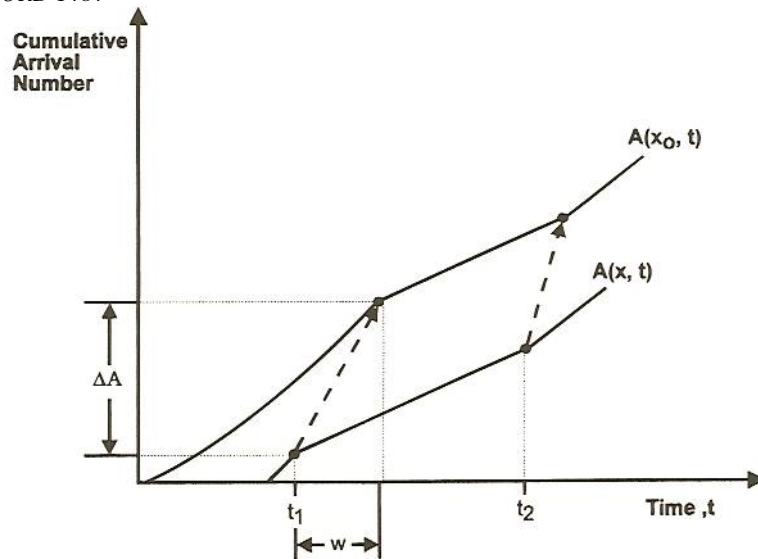
FIGURE 5 Backward-moving waves.
