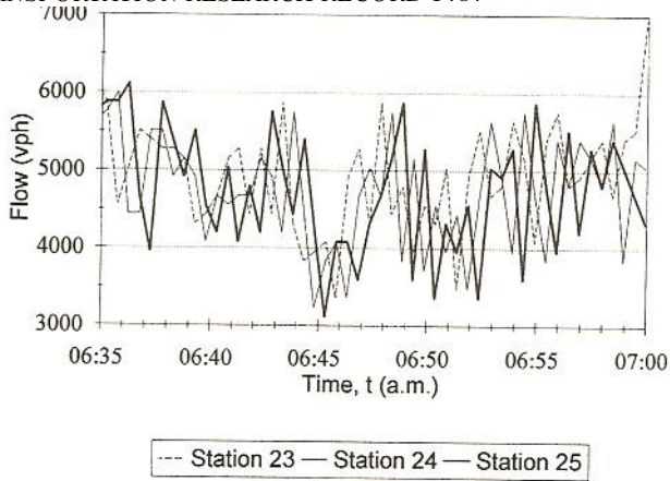
FIGURE 10 Time-series plot of 30-sec flows, Day 1.
