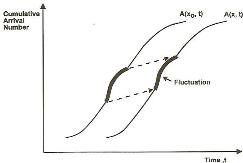
FIGURE 4 Wave propagating forward slower than vehicle speed.
