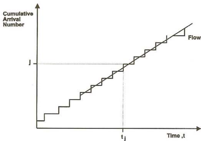
FIGURE 1 Cumulative vehicle arrival curve.
