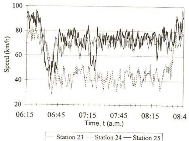
FIGURE 12 Measured speed profiles, Day 2.
