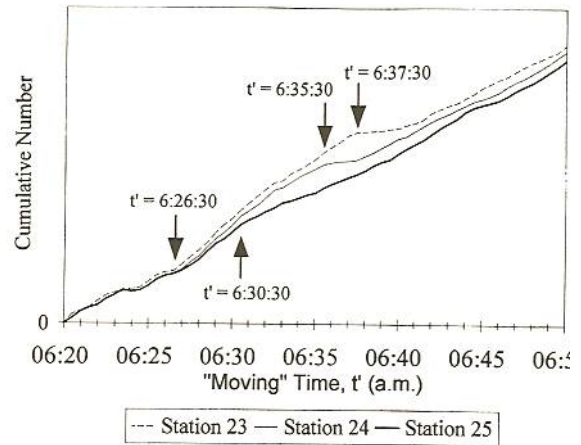
FIGURE 11 Backward-moving shock wave, Day 2.
